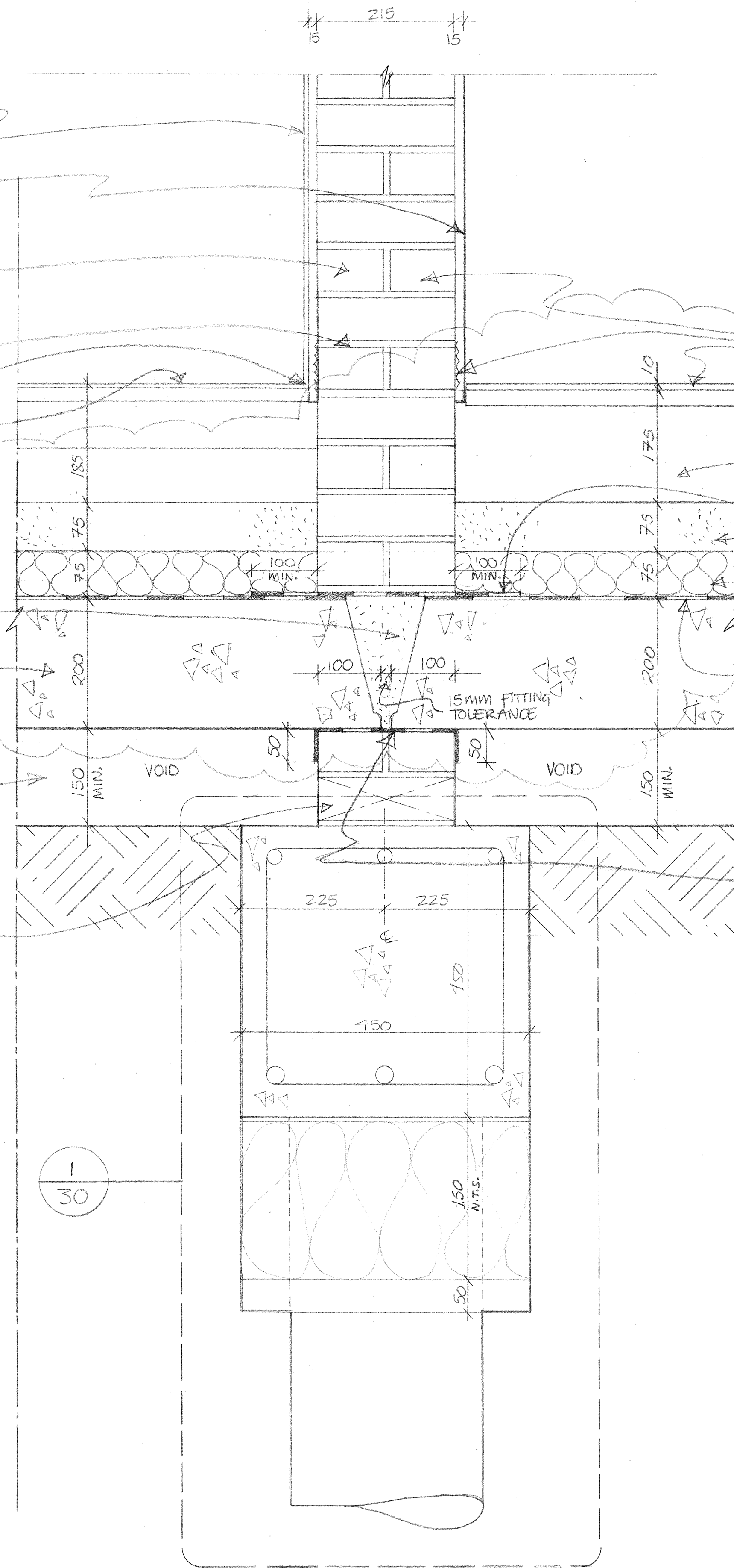
1/30 VERTICAL SECTION THROUGH 215MM BRICK WALL AT GROUND LEVEL (TYPICAL) 1:5
