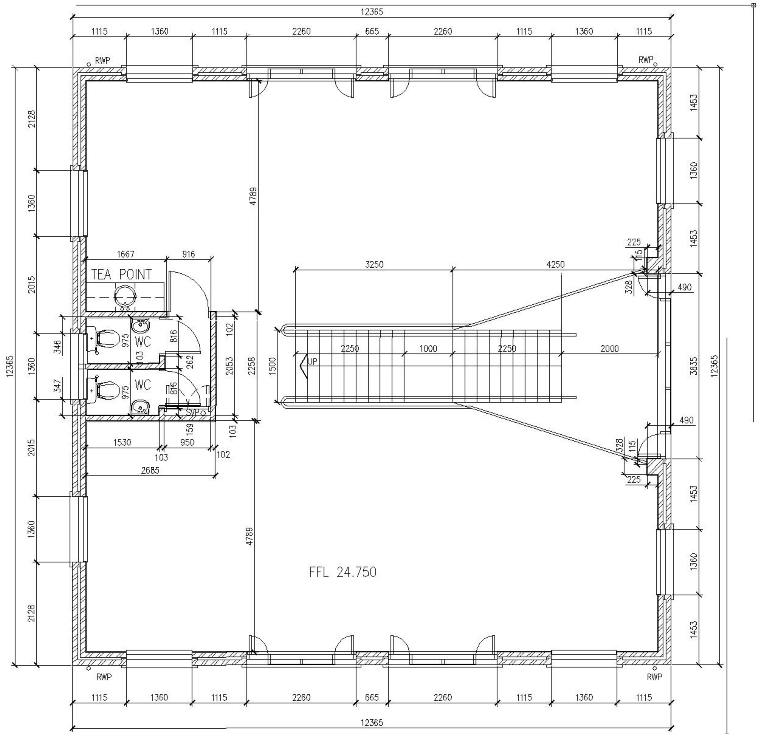
UNIT D FIRST FLOOR PLAN Scale 1:50
